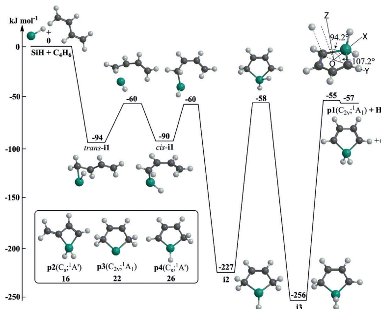
Figure 3. Potential energy surface of \text{SiC}_4\text{H}_7 for the reaction of the silyldyne radical with 1,3-butadiene leading to p1 (silole; \text{c-SiC}_4\text{H}_6 ) and atomic hydrogen. Three energetically accessible product isomers, p2–p4 , are shown along with the point groups and symmetries of the electronic wave functions. The energies are given in \text{kJ mol}^{-1} with respect to the initial reactant system. Carbon black, hydrogen light gray, silicon dark green.
